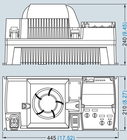
SINAMICS G110D, frame size FSC, with integrated line filter class A
