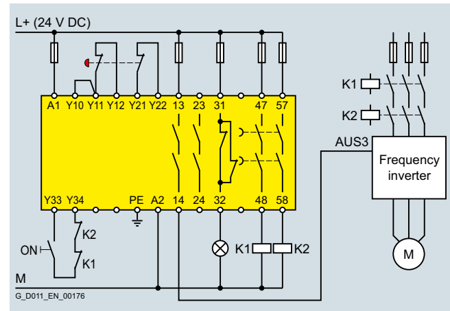
Conventional wiring
