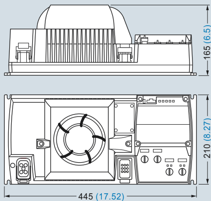
SINAMICS G110D, frame size FSB, with integrated line filter class A
