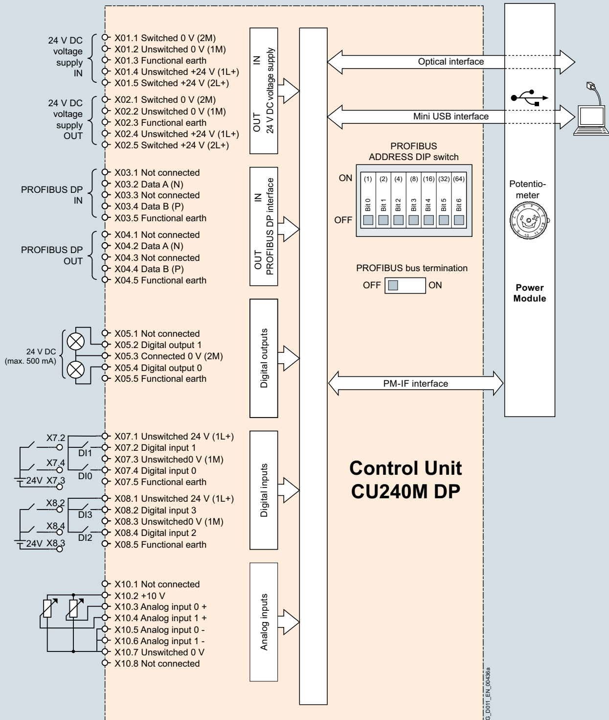
Connection diagram for CU240M DP Control Units
