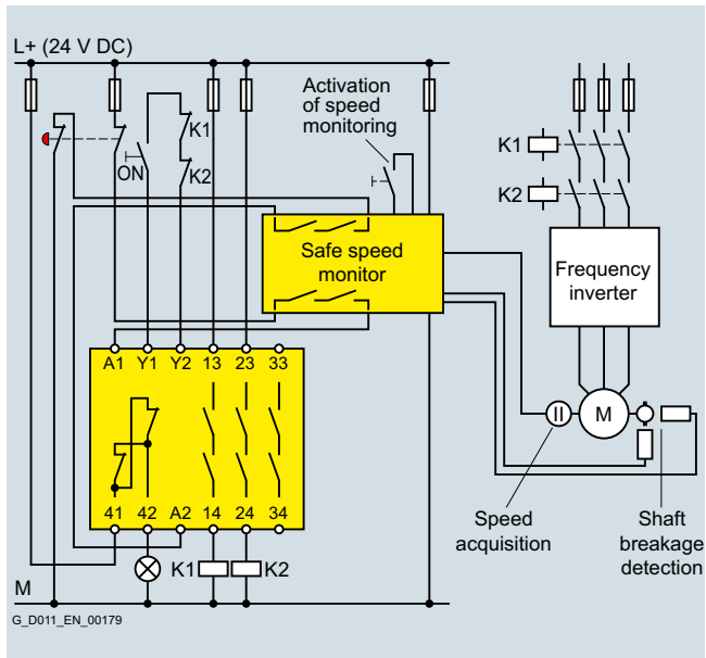
Conventional wiring
