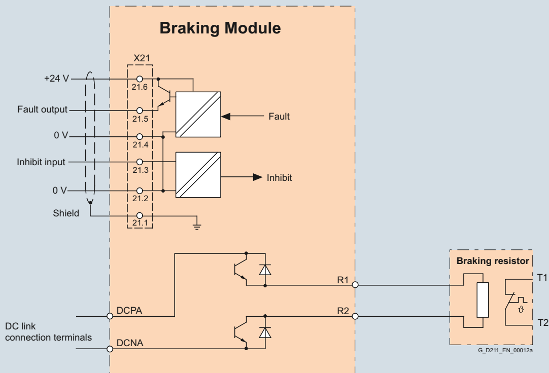
Connection example of a Braking Module
