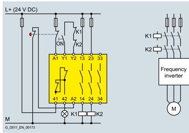
Conventional wiring
