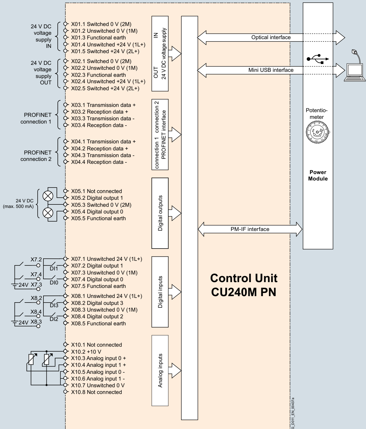
Connection diagram for CU240M PN Control Units
