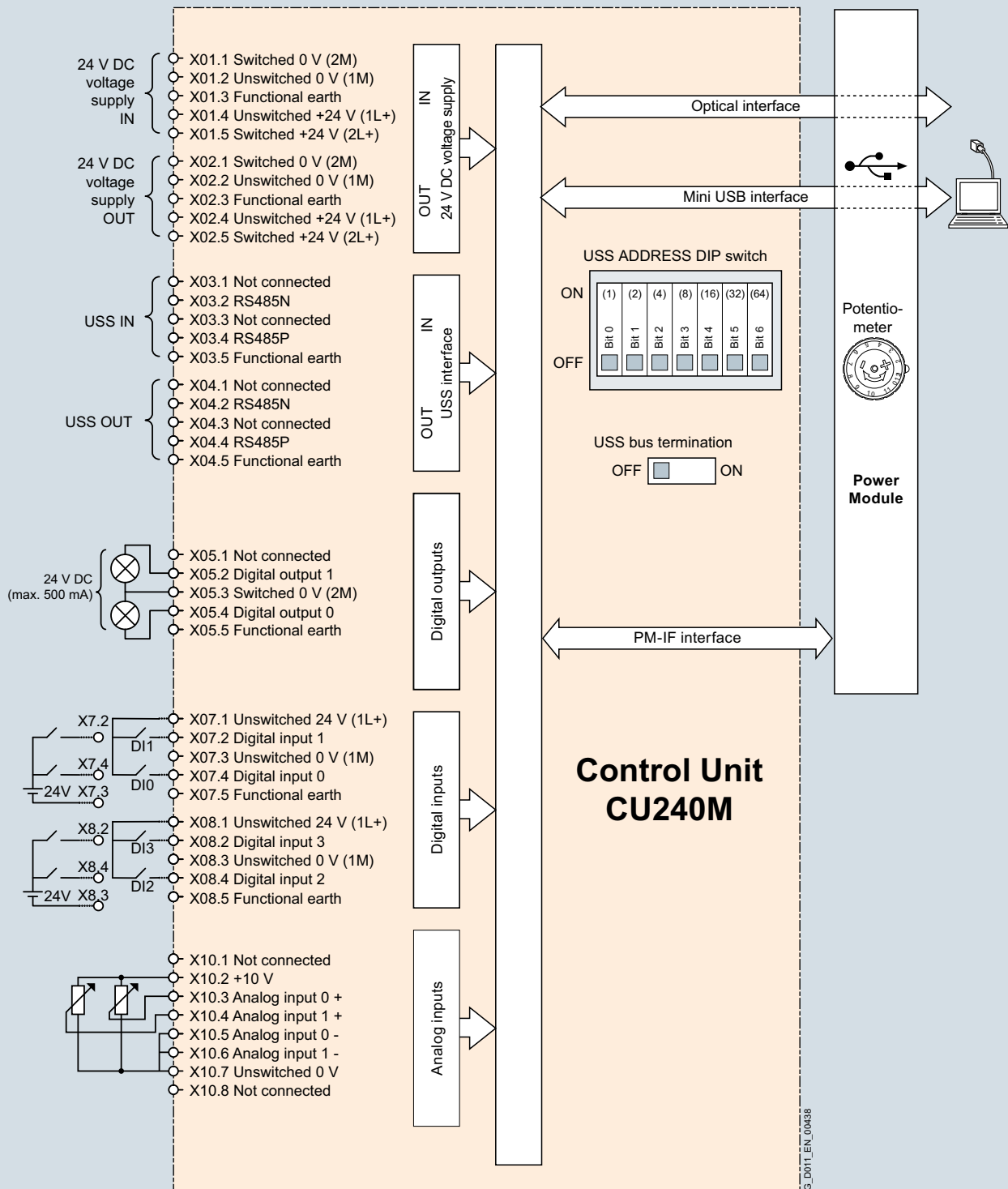
Connection diagram for CU240M Control Units
