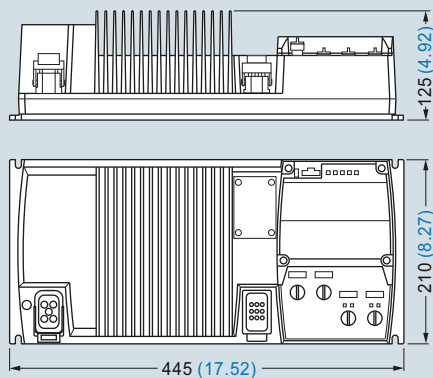
SINAMICS G110D, frame size FSA, with integrated line filter class A
