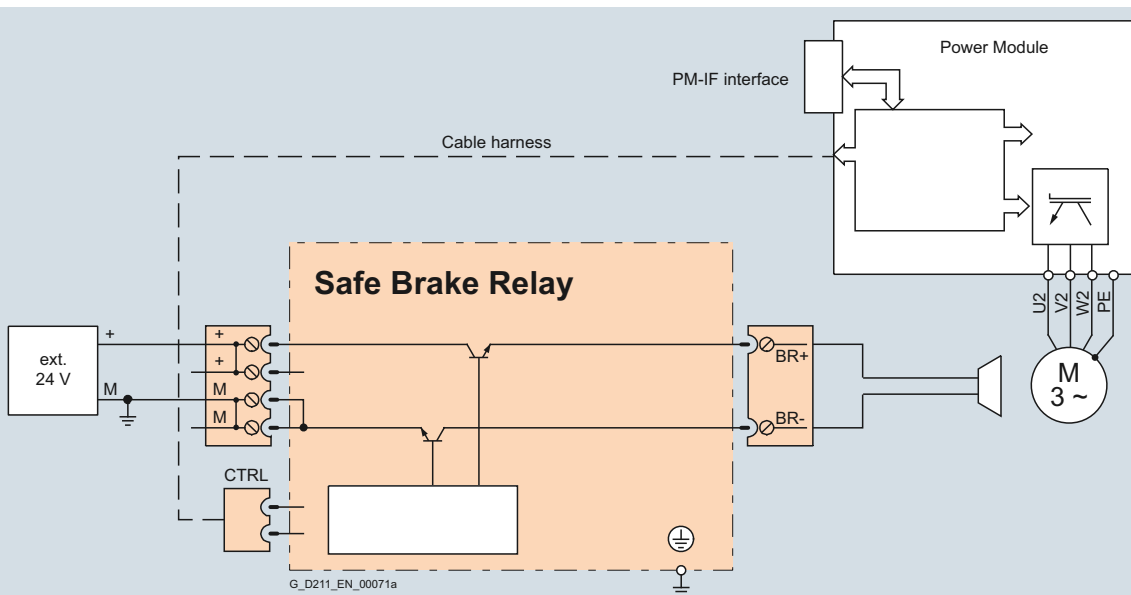
Connection example of Safe Brake Relay
